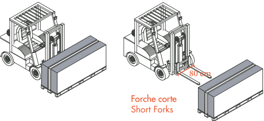
Carico su Camion Truck loading
